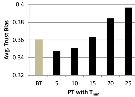
Fig. 5. Average trust bias of all nodes: PT vs. BT
