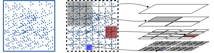
Fig. 1: 2D space decomposition (Quadtree). Grid view and hierarchical view.
