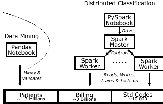
Figure 4: Architecture of Prediction System.
