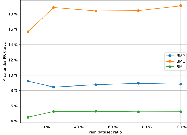
Figure 12: PR AUC (train subsets of varying sizes and same test subset), when predicting nosocomial infections. Notice that classes are heavily imbalanced since nosocomial infections occur for 3% of all admissions, and metrics are computed on a real (imbalanced) test subset.
