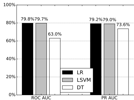
Figure 3: Comparison of Different Classifiers.
