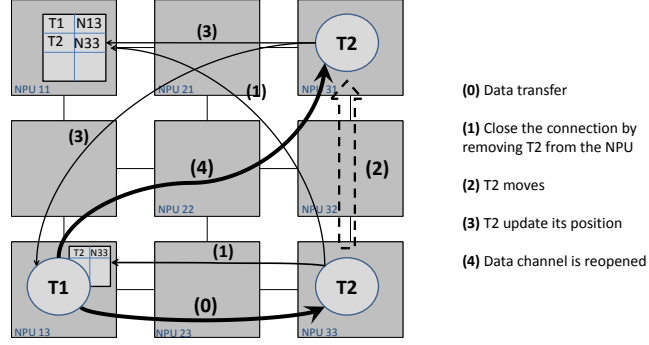
Fig. 8. First migration protocol
