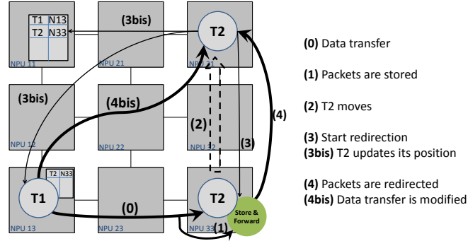
Fig. 10. Second migration protocol
