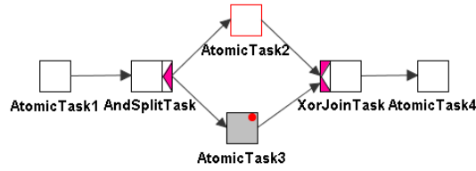
(b) YAWL
