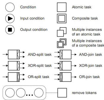
Figure 2. YAWL notations
