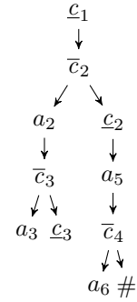
Fig. 3. Mapping \eta for a Word: c_1 \cdot \bar{c}_2 \cdot a_2 \cdot \bar{c}_3 \cdot a_3 \cdot \underline{c}_3 \cdot \bar{c}_2 \cdot a_5 \cdot \bar{c}_4 \cdot a_6 \cdot \# .
