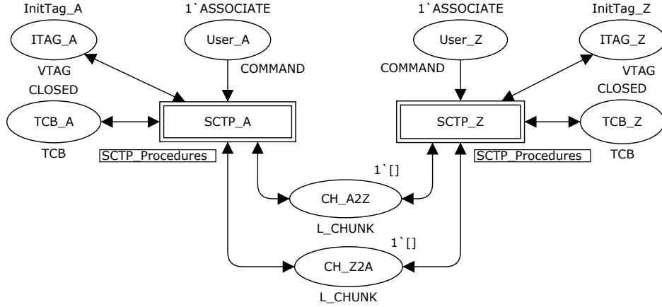
Fig. 4. The Top-level CPN page.
