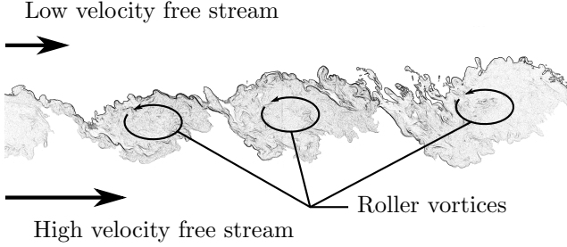
Fig. 1. Illustration of the organization of the turbulent mixing layer in the self-similar region (figure reproduced from Carlier and Sadjavi (2016)).
