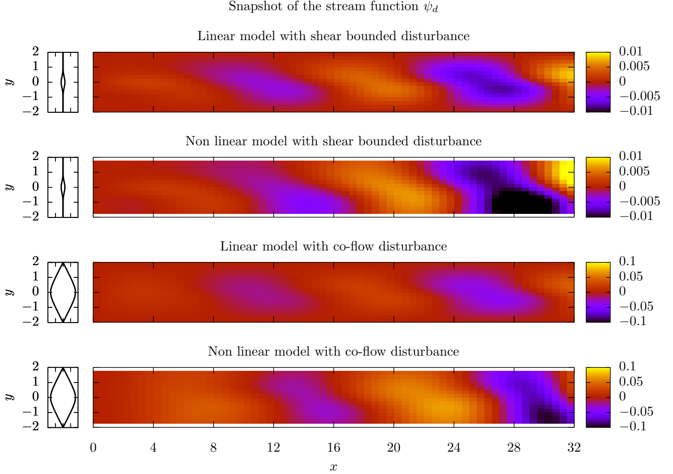
Fig. 5. Snapshots of the stream function \psi_d : Comparison between linear and non linear model for two kinds of input disturbances with sinusoidal amplitude.
