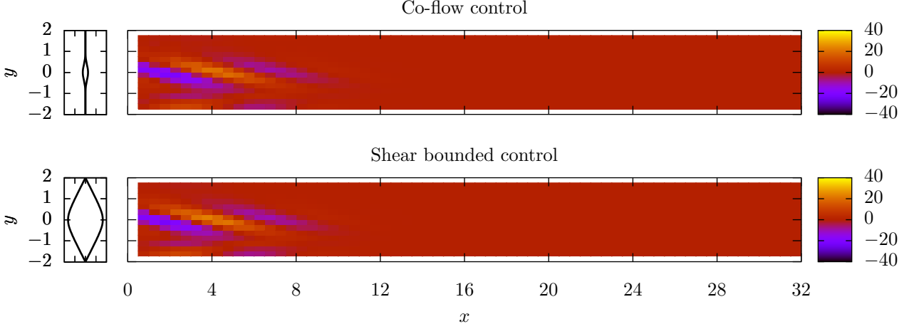
Fig. 4. Spatial distribution of the feedback gain \mathbf{K} .
