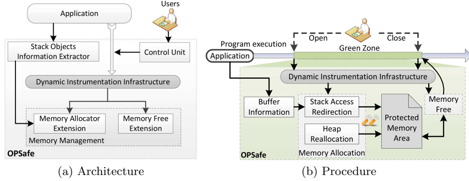
Fig. 1. OPSafe Design
