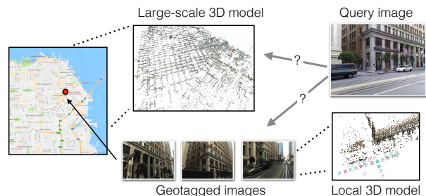
Figure 1. The state-of-the-art for large-scale visual localization. 2D image-based methods (bottom) use image retrieval and return the pose of the most relevant database image. 3D structure-based methods (top) use 2D-3D matches against a 3D model for camera pose estimation. Both approaches have been developed largely independently of each other and never compared properly before.
