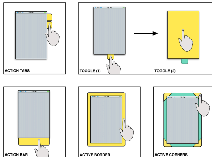
Figure 5: Action controllers
