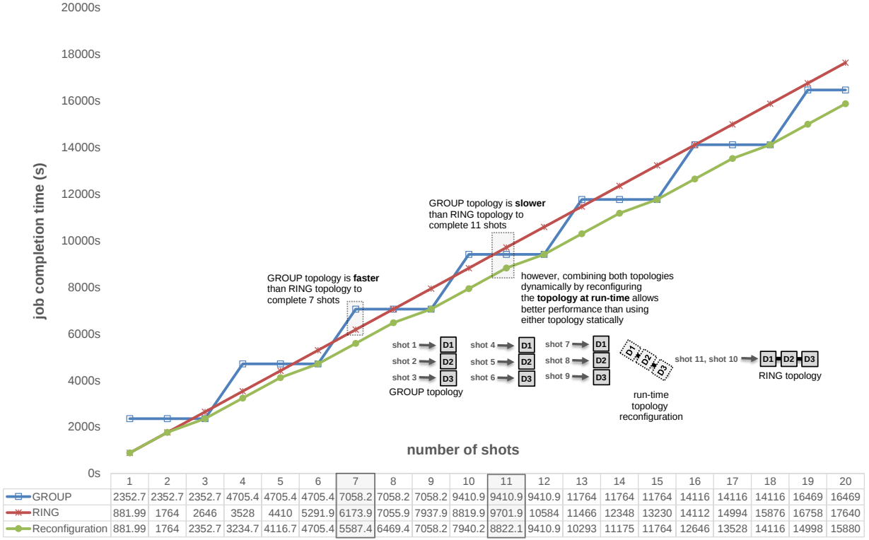
Figure 11: The effect of different DFE topologies on RTM performance.
