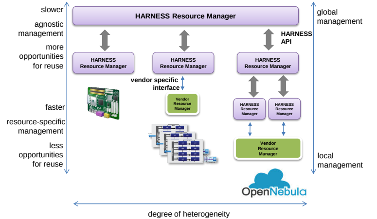
Figure 2: A heterogeneous cloud computing platform, supporting various types of resources, can be built by composing resource managers that implement the HARNESS API in a hierarchical system.
