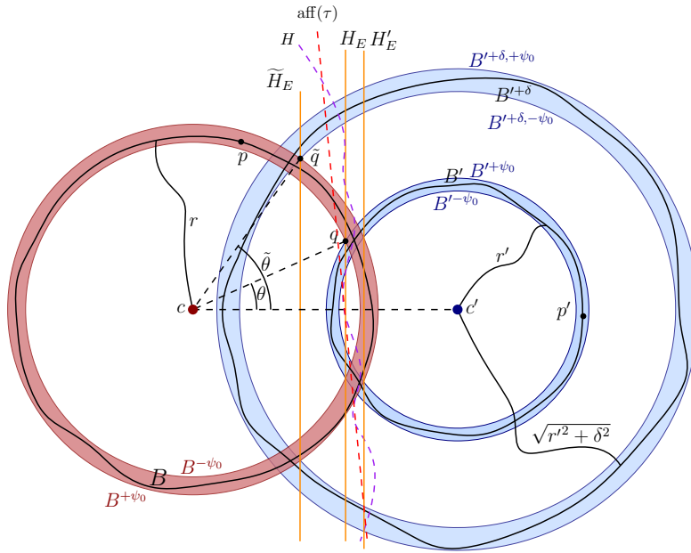
Figure 10: Construction and notations used in the proof of Lemma D.5
