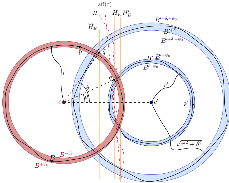
Figure 10: Construction and notations used in the proof of Lemma D.5
