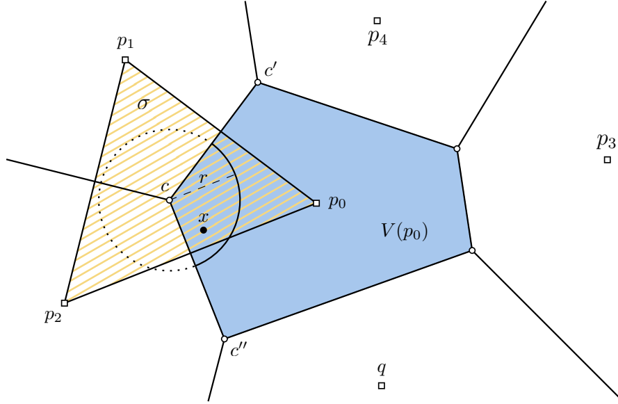
Figure 8: Illustration of the notations for the proof of Lemma 6.5. The simplex \sigma is dashed in yellow and has vertices p_0p_1p_2 . The distances cc' and cc'' are lower bounded by \delta^2/4\varepsilon .
