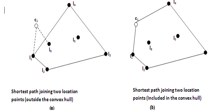
Fig. 2: Counter example
