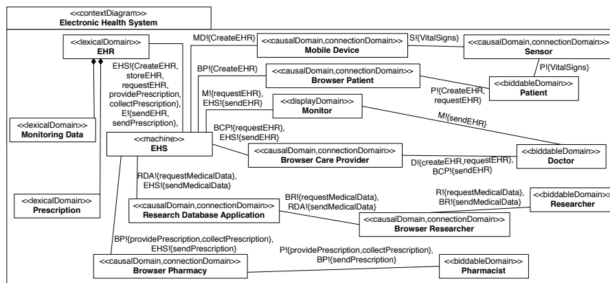
Fig. 5: Context Diagram
