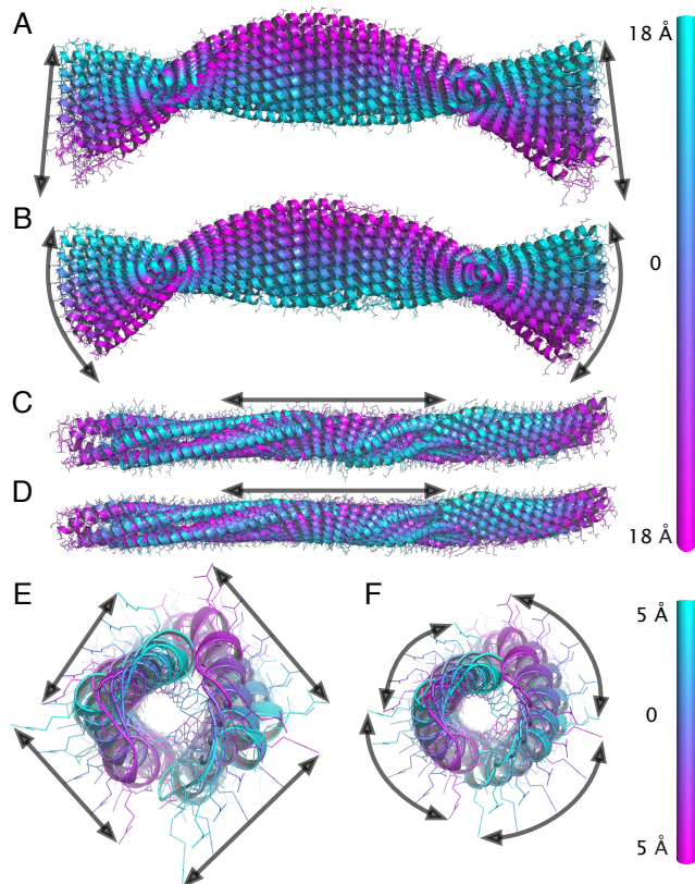
Figure 2: Comparison of linear (A, C, E) and non-linear (B, D, F) motion extrapolations of a coiled coil protein (pdb code 2ch7). Three types of motions are shown, bending (A, B), stretching (C, D), and twisting (E, F). Several snapshots at different deformation amplitudes are superposed to each other. These are colored according to the values of the overall deformation, as measured by the root-mean-square deviation (RMSD) . The colorbars show the RMSD with respect to the initial position. The arrows follow the trajectories of individual atoms.
