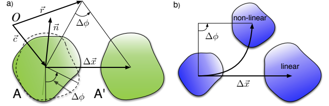
Figure 1: A motion of a rigid block. a) A rigid block A with the COM at \vec{c} is rotated about an axis \vec{n} by an angle \Delta\phi , and then translated by a vector \Delta\vec{x} . The result of the first rotation is shown as a dashed outline. The result of the complete motion is denoted as A'. This motion can be also represented as a pure rotation about a new center \vec{r} by the same angle \Delta\phi . The origin of the coordinate system is denoted as O. b) Schematic comparison of the linear and non-linear motion extrapolation methods. Please notice the final positions of the centers of mass and the size of the rigid blocks.
