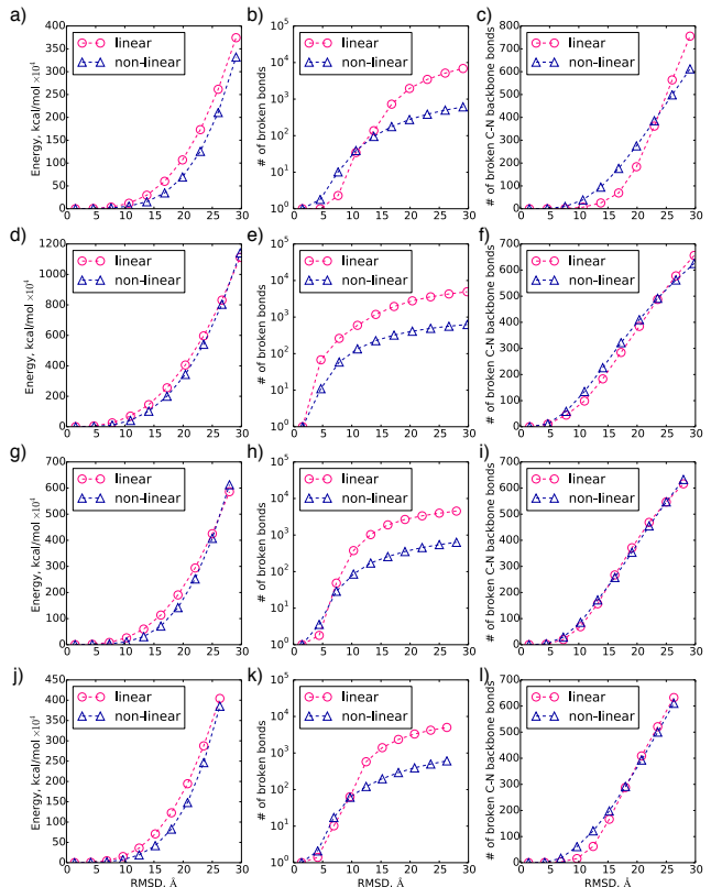
Figure 4: Comparison of linear and non-linear deformations averaged over the 10 lowest normal modes computed for the following systems, (a-c) 4bij, (d-f) 5a63, (g-i) 3j9j, and (j-l) 3j5p. In (a,d,g,j) the bond harmonic energy as a function of the deformation amplitude is shown. In (b,e,h,k) the total number of broken bonds as a function of the deformation amplitude is shown (in a log scale). In (c,f,i,l) the number of broken bonds between individual amino acids is shown as a function of the deformation amplitude. See the main text for details.
