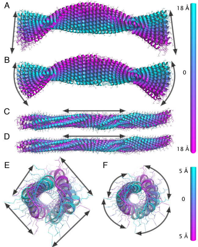
Figure 2: Comparison of linear (A, C, E) and non-linear (B, D, F) motion extrapolations of a coiled coil protein (pdb code 2ch7). Three types of motions are shown, bending (A, B), stretching (C, D), and twisting (E, F). Several snapshots at different deformation amplitudes are superposed to each other. These are colored according to the values of the overall deformation, as measured by the root-mean-square deviation (RMSD) . The colorbars show the RMSD with respect to the initial position. The arrows follow the trajectories of individual atoms.
