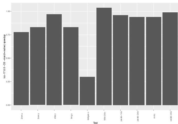
PolyBench, test icc -O3
