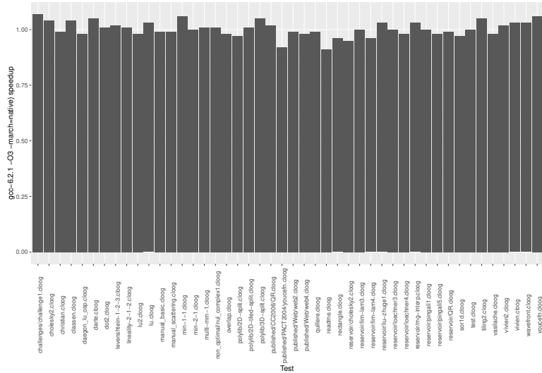
CLoG test suite, gcc -O3
