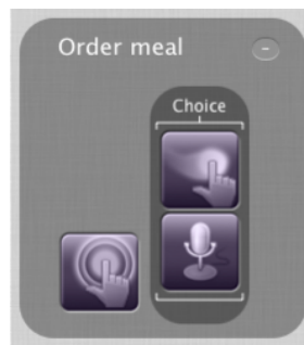
Fig. 8. Detail of the post-WIMP layer: More complex post-WIMP interactions can be created by combining single gestures or events. In this case, a long press combined with either a swipe or voice input form a combined post-WIMP element, which can be connected to an action.
