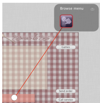
Fig. 6. Detail of the post-WIMP layer: A newly created pan gesture is being displayed in a small box. After connecting the pan to the area where it can be executed (“activity area”), the respective region shows a red overlay. A red frame around the pan symbol indicates that it has been connected to an activity area.
