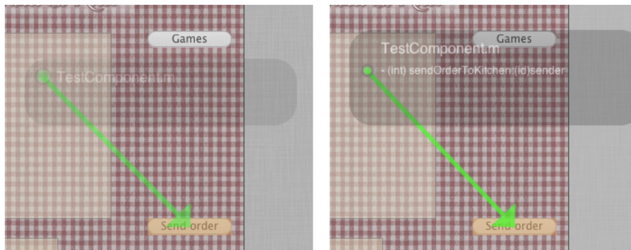
Fig. 5. Two phases of the transition from GUI layer to code layer: A small pop-up first displays the source file only (left image), then also the method the selected GUI button is connected to (right image).
