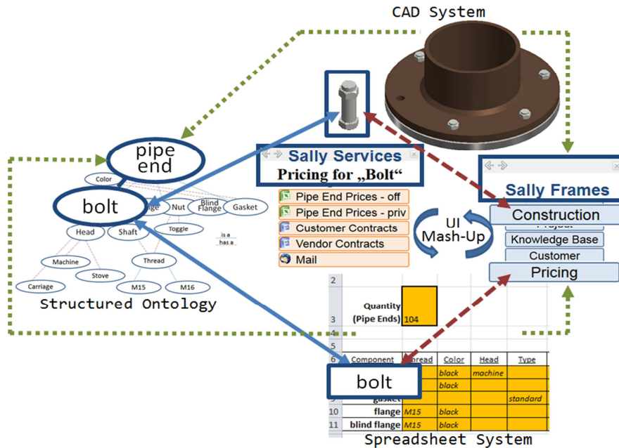
Fig. 5. Mashup of Interfaces
