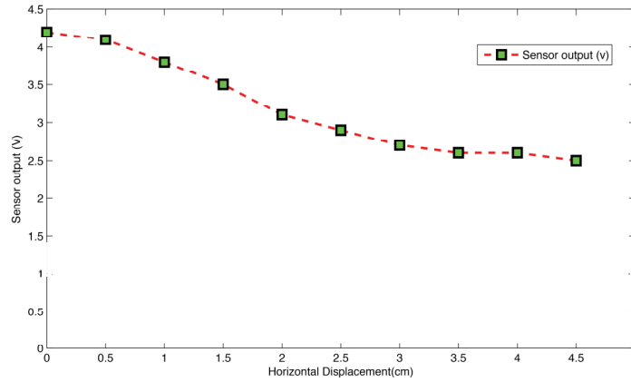
Fig.6. Hall Effect sensor output versus horizontal displacement.
