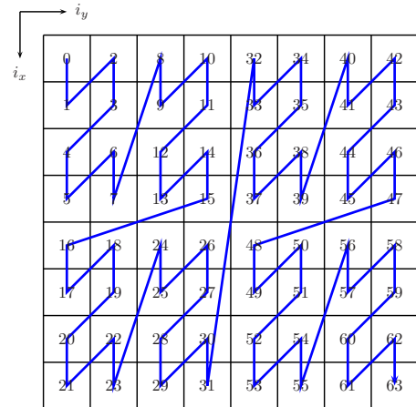
Figure 3. Morton layout of a 8 x 8 matrix.
