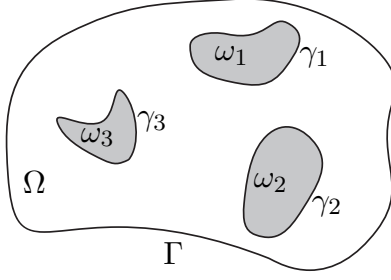
Figure 1: The multiply connected cavity.
