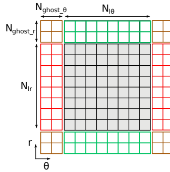
Figure 4: Halo size of a r \times \theta subdomain. The local points of the subdomain are in gray.
