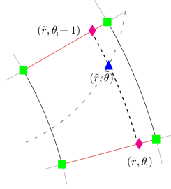
Figure 2: Second step of the bi-dimensional interpolation. \blacktriangle is the target point and the intermediate points \blacklozenge are obtained by interpolating the two corners \blacksquare of their respective red edges with Hermite scheme.
