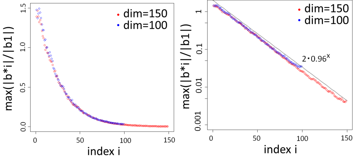
Fig. 5. Evolution of \max_B \|\mathbf{b}_i^*\| / \|\mathbf{b}_1\| over hundreds thousands LLL-reduced bases, as i \geq 2 increases, in dimensions 100 (blue) and 150 (red): the right-hand graph is in log-scale.
