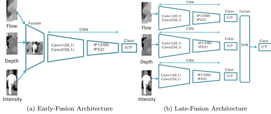
Fig. 1: Stereo Vision Modality Fusion Architectures. \text{Conv}(f,s) represents a convolution layer with f filters and a stride of s .
