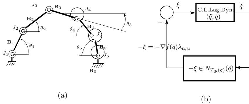
Fig. 7: (a) Clearances at J_4 , J_5 and J_6 . (b) Interconnected closed-loop in (45).
