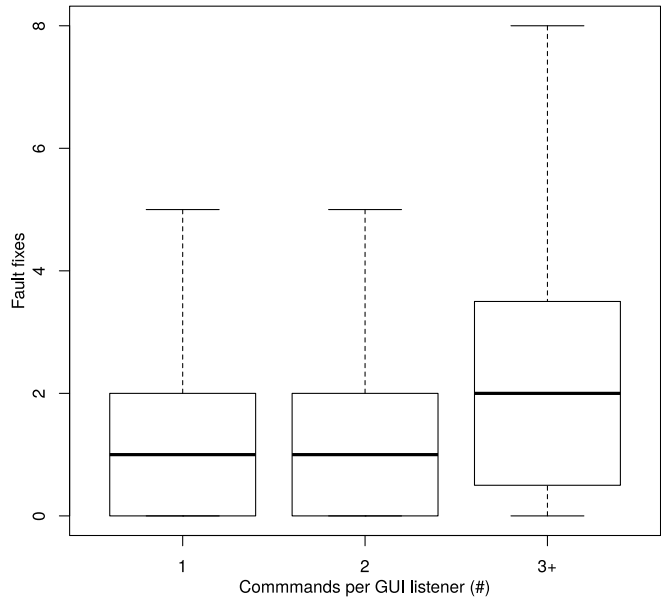
Figure 3: Number of fault fixes of UI listeners
