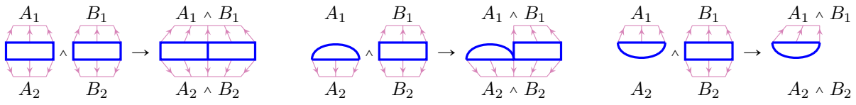
Figure 2. Conjunction of simple combinatorial flows
