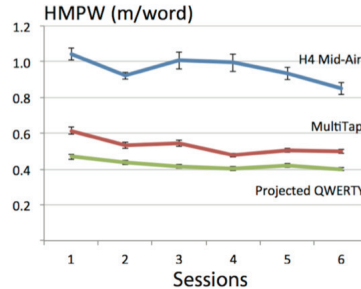
Fig. 9. Mean HMPW for the three text entry methods over sessions. Error bars show standard error of the mean.
