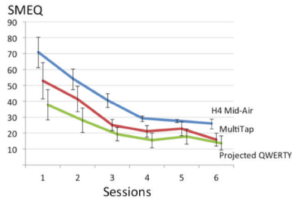
Fig. 8. Mean SMEQ scores over sessions for the three text entry methods. Error bars show standard error of the mean.
