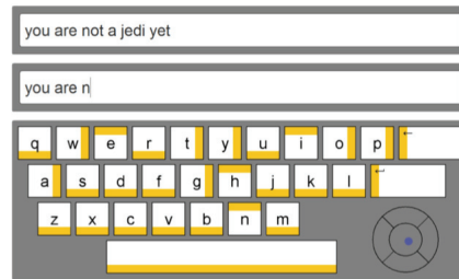
Fig. 2. The user interface for H4 Mid-Air.
