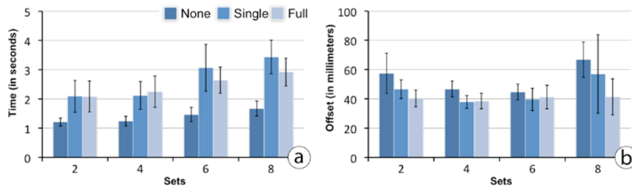
Fig. 6. Results of the placement study: (a) retrieval time for one item for all feedback conditions and sets; (b) offset for correct retrievals measured as Euclidean distance between the item's center and the touch's location. Error bars represent 95% confidence intervals.
