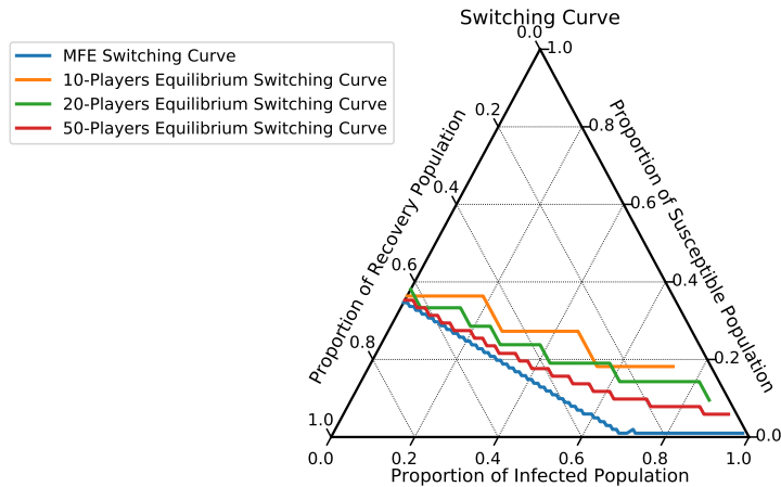
Figure 5: Convergence of the Nash switching curve to to the MFE switching curve
