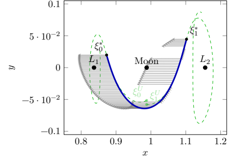
(b) Optimal solutions for the transfer between the two invariant manifolds. The solutions for the minimization of the L^2 -norm of the control and the solution for the L^1 -norm overlap because of the tiny difference between them.
