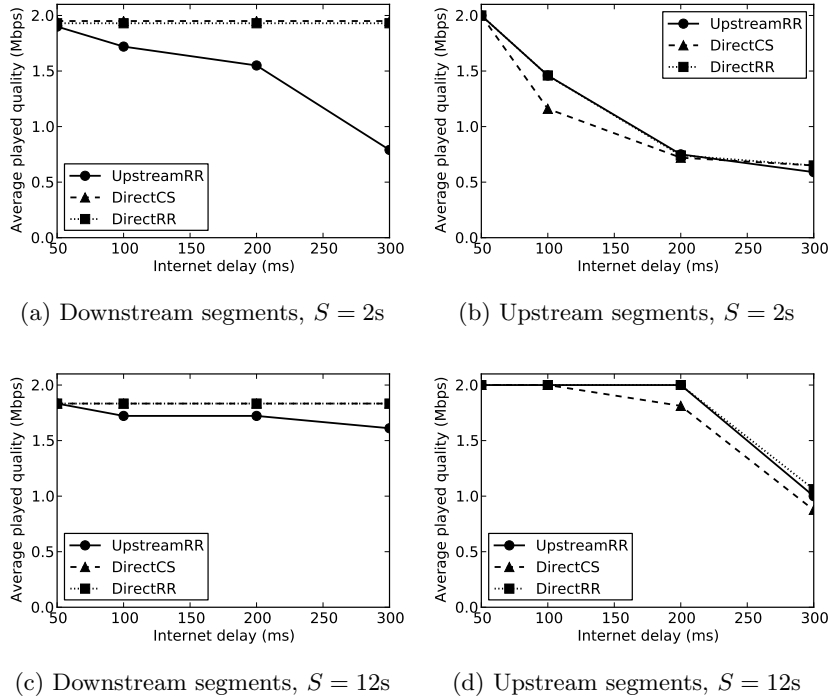
Fig. 6: The average played quality as a function of one-way Internet delay ID , for different values of segment duration S ; for DD = 5\text{ms} , B = 5\text{Mbps} , and P = 36\text{s}
