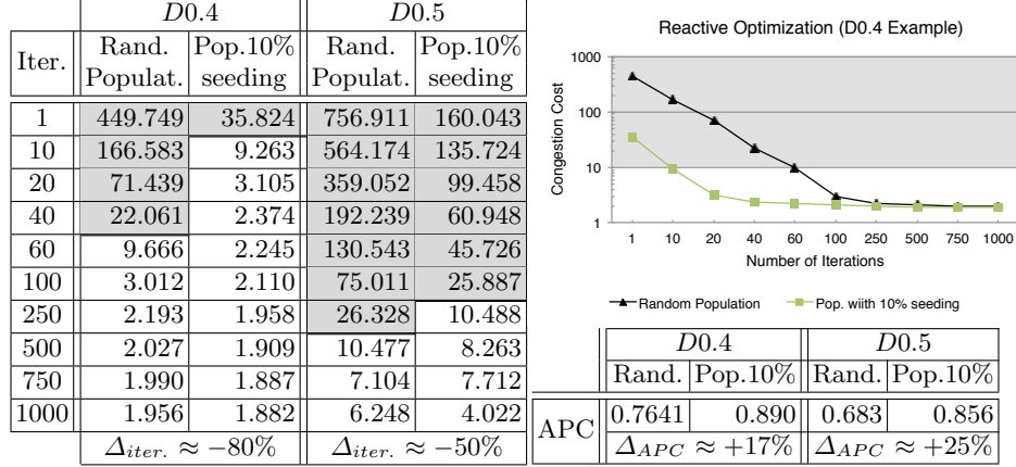
Fig. 2. Reactive link failure optimization: Iterations and APC metric (D0.4, D0.5)
