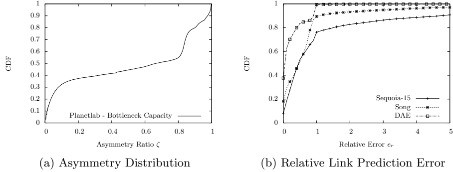
Fig. 5: PlanetLab Topology
