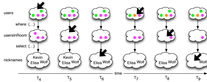
Fig. 2. Removing a user from the ambient cloud and changing the chatroom attribute of a user
