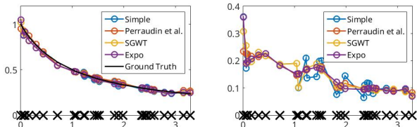
Fig. 4: Comparison of PSD estimators on the GMRF model (left) and the temperature dataset (right).
