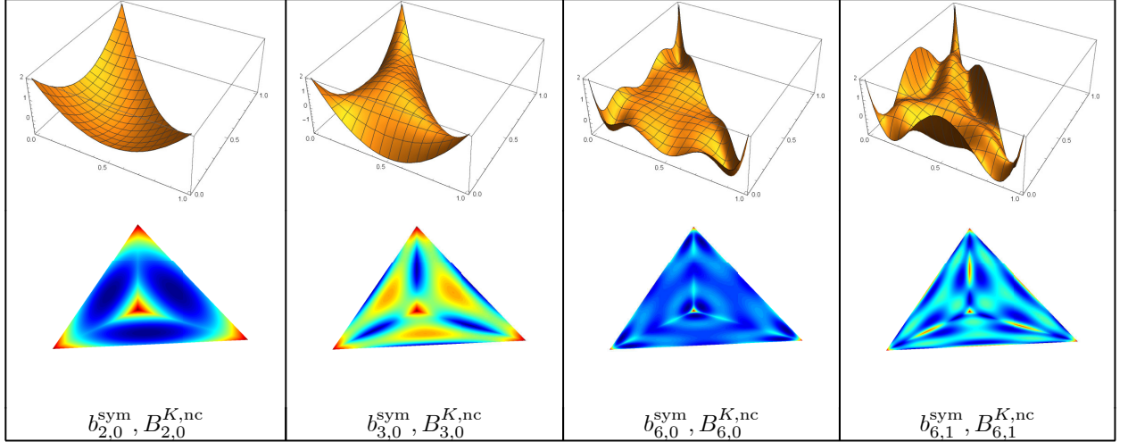
Figure 1: Symmetric orthogonal polynomials on the reference triangle and corresponding tetrahedron-supported non-conforming basis functions.
