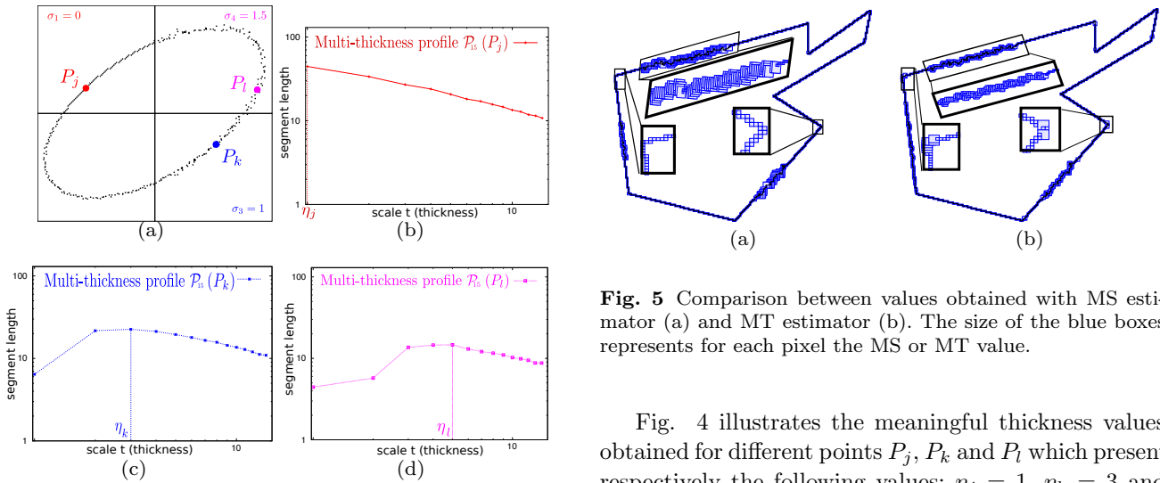
Fig. 4 Multi-thickness profiles (b-d) obtained on different points: P_j with no noise (graph (b)), with low noise ( P_k , graph (c)) and important noise ( P_l , graph (d)). The meaningful thickness values \eta_j , \eta_k and \eta_l are represented on each multi-thickness profile \mathcal{P}_{15} .
