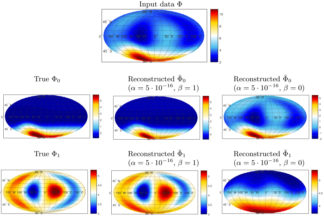
Figure 5: Results for radii R_1 = 0.5 , R_0 = 1 , and R_2 = 1.06 : Input data \Phi = \Phi_0 + \Phi_1 (top), ground truth \Phi_0 , \Phi_1 (bottom left), reconstructed \bar{\Phi}_0 , \bar{\Phi}_1 with localization constraint (bottom center), and reconstructed \bar{\Phi}_0 , \bar{\Phi}_1 without localization constraint (bottom right).
