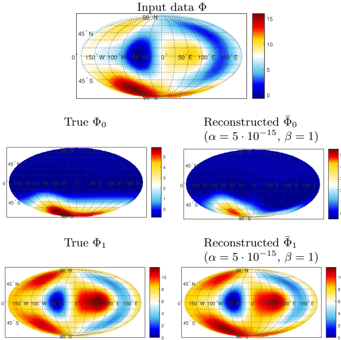
Figure 6: Results for radii R_1 = 0.8 , R_0 = 1 , and R_2 = 1.06 : Input data \Phi = \Phi_0 + \Phi_1 (top), ground truth \Phi_0 , \Phi_1 (bottom left), and reconstructed \bar{\Phi}_0 , \bar{\Phi}_1 with localization constraint (bottom right).
