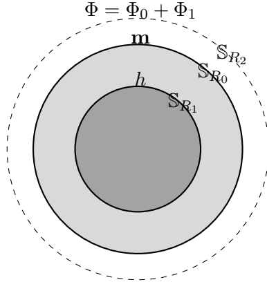
Figure 1: Illustration of the setup of Problem 1.1.
