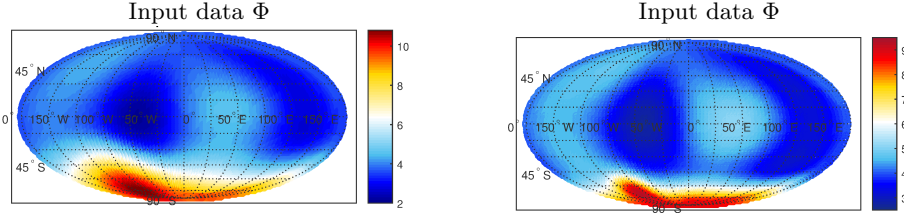
Figure 2: Spatial plot of the input data \Phi with parameters \gamma_1 = \frac{1}{20} , \gamma_2 = \frac{1}{2} (left) and \gamma_1 = \frac{3}{5} , \gamma_2 = \frac{3}{5} (right) for the magnetization \mathbf{m} from (5.10).
