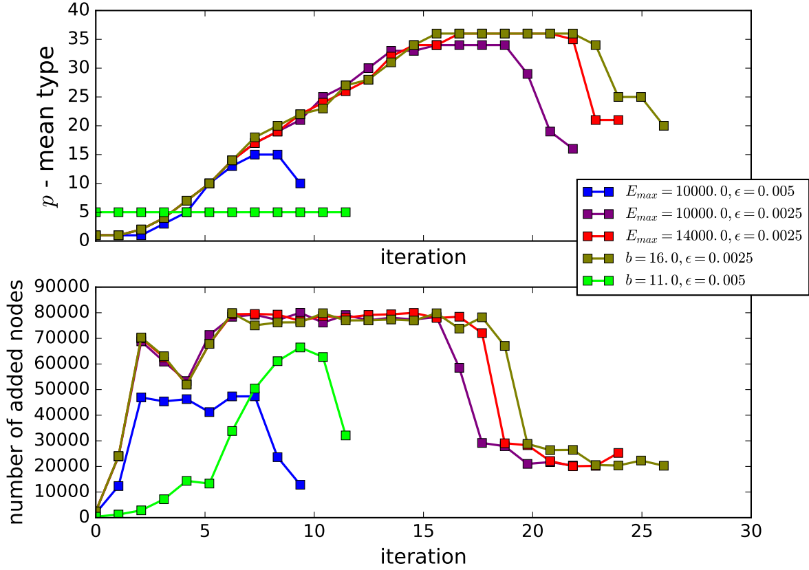
Figure 3: Evolution of the average type p during the A-VCI iterations for C_2H_4O ( F = 50 ). The basis expansion strategy is aCCW, except for the green curve obtained with CCW(5). The used approximation spaces are \Pi_d(E_{max}) and BP(b) .
