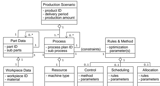
Fig. 6. - Structure of a production scenario[8]
