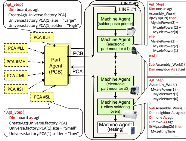
Fig. 12. - Modelling of the PCA production line
