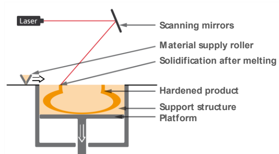
Fig. 1. Schematic diagram of SLS [following VDI 3404]
