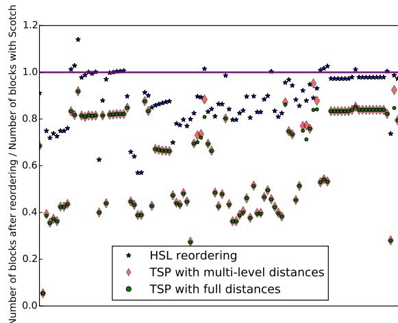
Fig. 10: Impact of the heuristic used on the ratio of off-diagonal blocks over those produced by the initial SCOTCH ordering on the Florida set of matrices. The lower the better.
