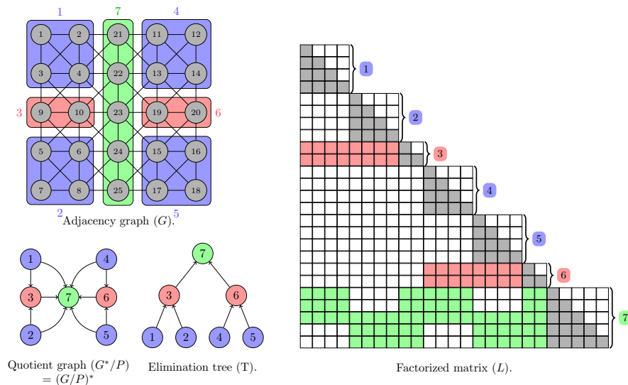
Fig. 1: Nested dissection and block-data structure for L .
