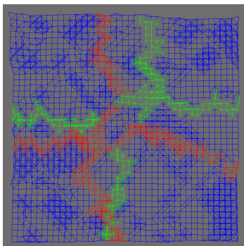
Fig. 6: Projection of contributing supernodes on the first separator of a 3D laplacian of size 40 \times 40 \times 40 , using SCOTCH.
