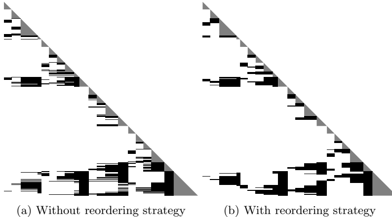
Fig. 8: Block-symbolic factorization of 8 \times 8 \times 8 Laplacian initially reordered with SCOTCH.
