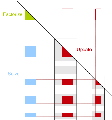
Fig. 2: Steps to factorize the matrix - symmetric positive definite case.
