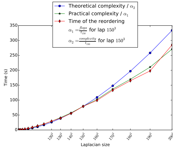
Fig. 9: Comparison of the time of reordering against theoretical and practical complexities on 3D Laplacians.
