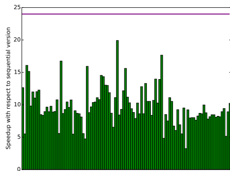
Fig. 12: Speedup of the reordering step (full distance heuristic) with 24 threads on the full set of matrices.
