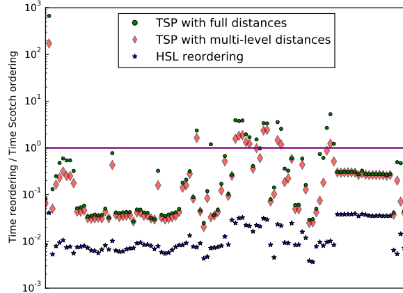
Fig. 11: Time of the sequential reordering step with respect to the initial SCOTCH ordering on the Florida set of matrices. The lower the better.
