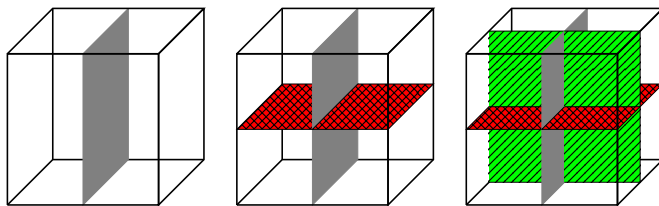
Fig. 3: Three-levels of nested dissection on a regular cube.
