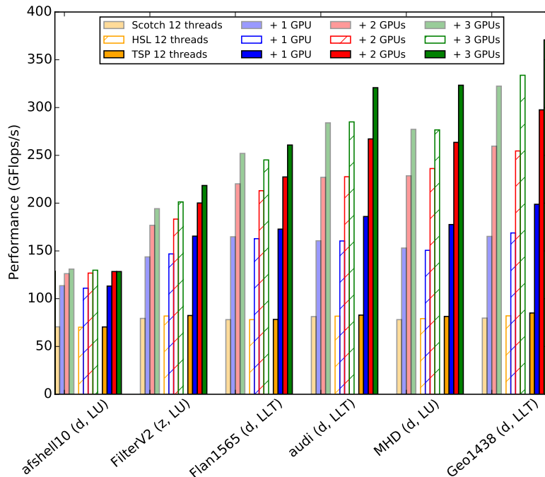
Fig. 13: Performance impact of the reordering algorithms on the PASTIX solver on top of the PARSEC runtime with 1 node of the hybrid mirage architecture.
