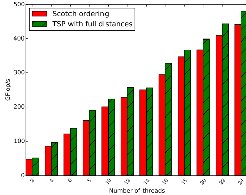
Fig. 14: Scalability on the CEA 10 million unknowns matrix with 24 threads.
