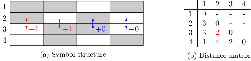
Fig. 7: Example of a symbolic structure and its associated distance matrix. Computation of the distance between rows 2 and 3 is illustrated.
