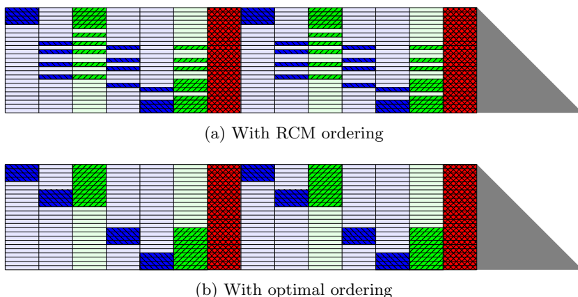
Fig. 5: Off-diagonal blocks contributing to the first separator in figure 3.
