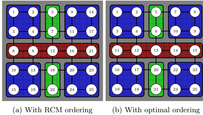
Fig. 4: Projection of contributing supernodes and ordering on the first separator (gray in figure 3).
