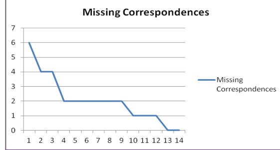
Fig. 6. Missing Correspondences
