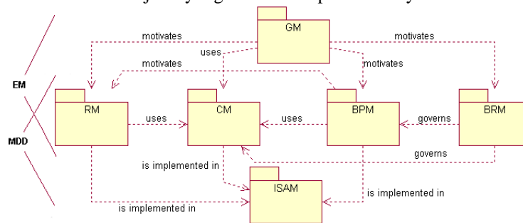
Fig. 1. The Complimentary Views of the Unifying Meta-Model.
